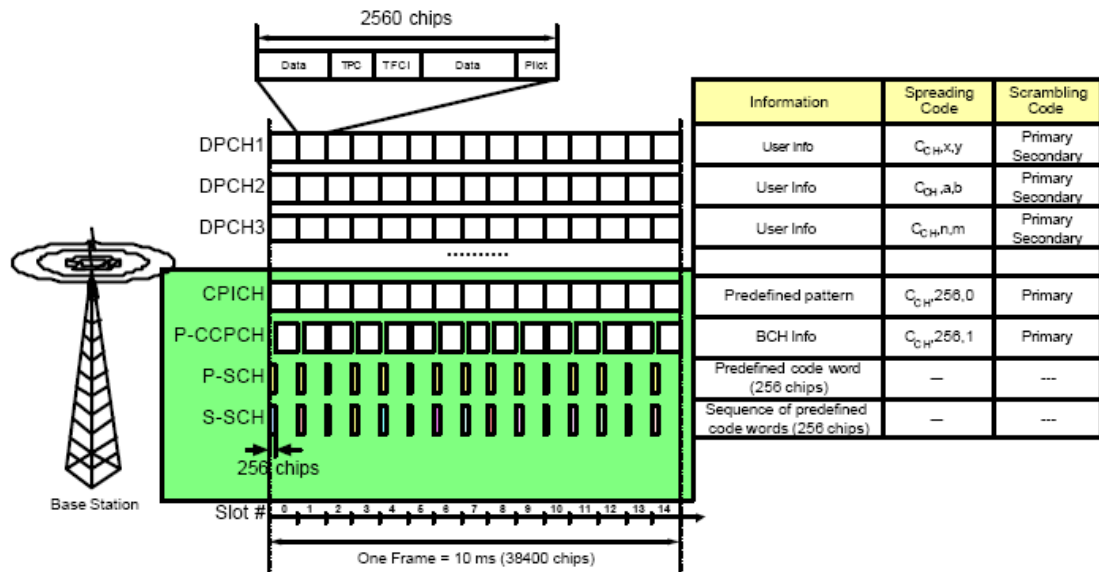
Physical channels used for synchronisation
